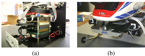
Fig. 3. (a) Photo of PC/104+ stack out of box; the left lower panel holds the Firewire connectors; CPU resides on top. (b) Stereo camera mount; cameras rotated upwards for picture only.
