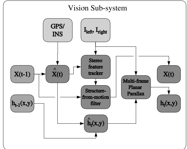
Fig. 2. The architecture of the vision sub-system.
